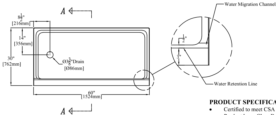
60" x 30" [1524mm x 762mm] Shower Pan w/ 8" [203mm] Threshold
