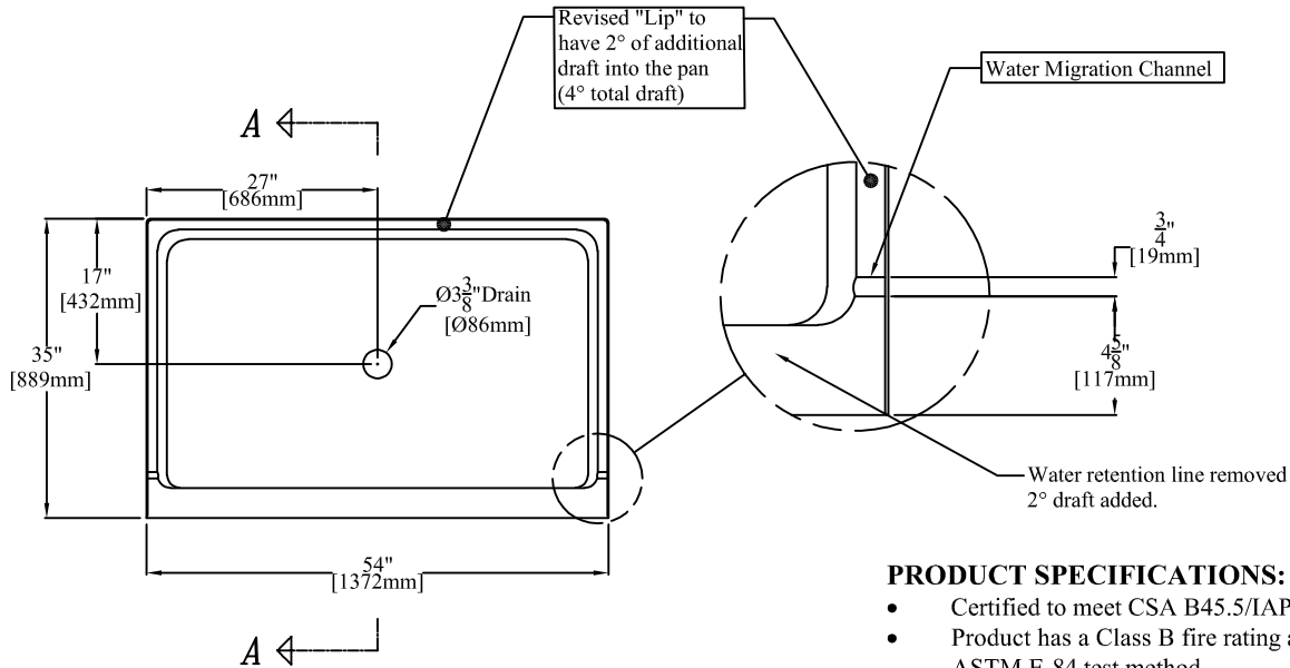
54" x 35" [1372mm x 889mm] Shower Pan w/ 6" [152mm] Threshold
