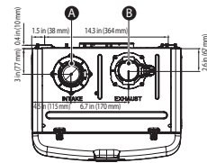
Overhead View
