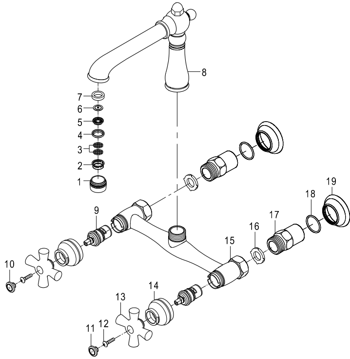
Cold Handle: KSH3221PXC
