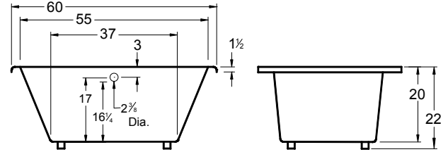
All bathtub dimensions are \pm 1/2"
